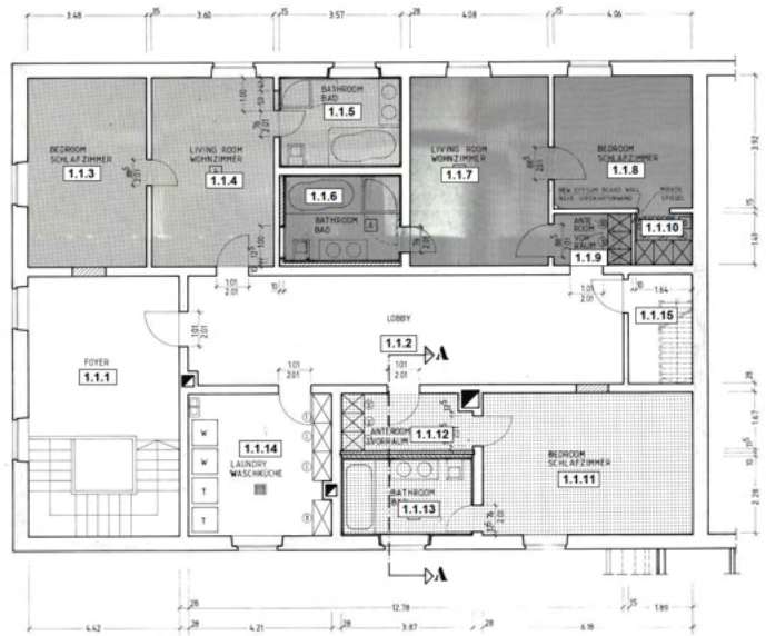
SECOND FLOOR, NEW OBERGESCHOSS, NEU 1:50
