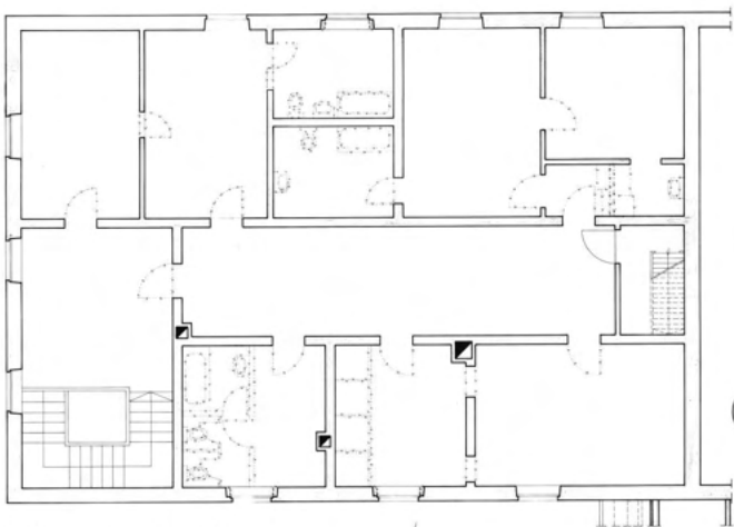
SECOND FLOOR, DEMOLITION OBERGESCHOSS, ABRUCH 1:50
